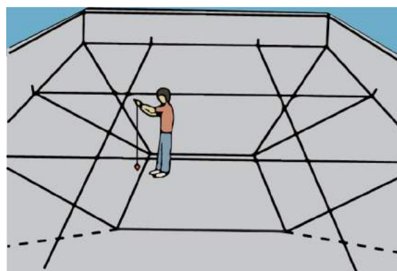
HOPPER STAKES AT INTERSECTION OF STRINGS
