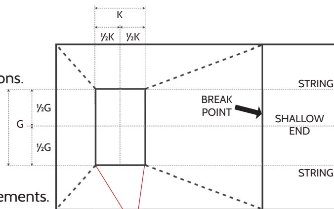
HOPPER STAKES AT INTERSECTION OF STRINGS
